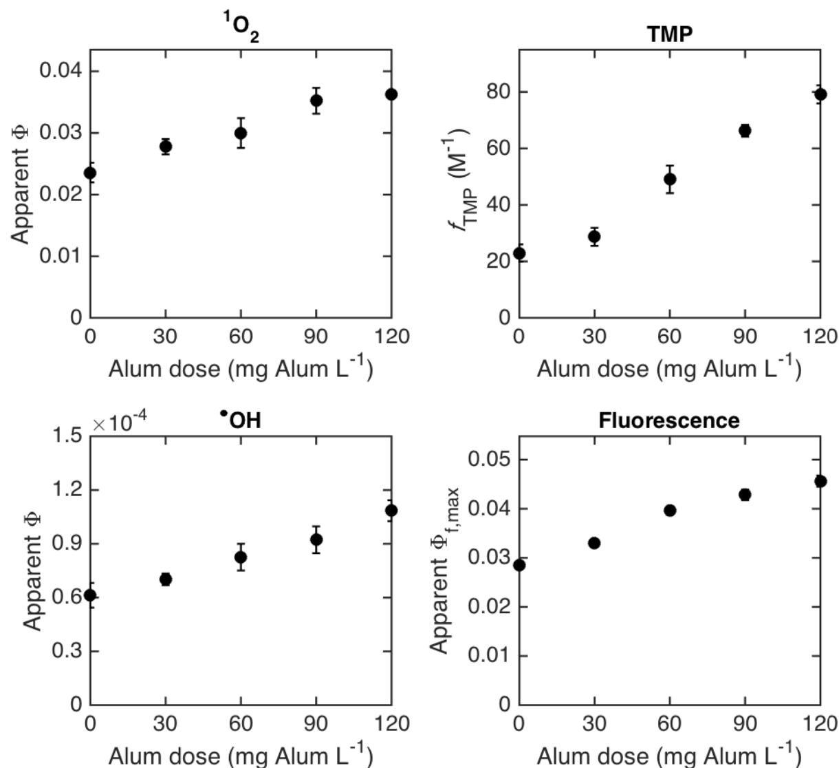
Figure 3.4. Apparent quantum yields for 1 O 2 , •OH, fluorescence, and TMP degradation efficiencies for LM wastewater pre- and post-coagulation with Alum. Data points are averages of duplicate runs and error bars represent two standard deviations.
