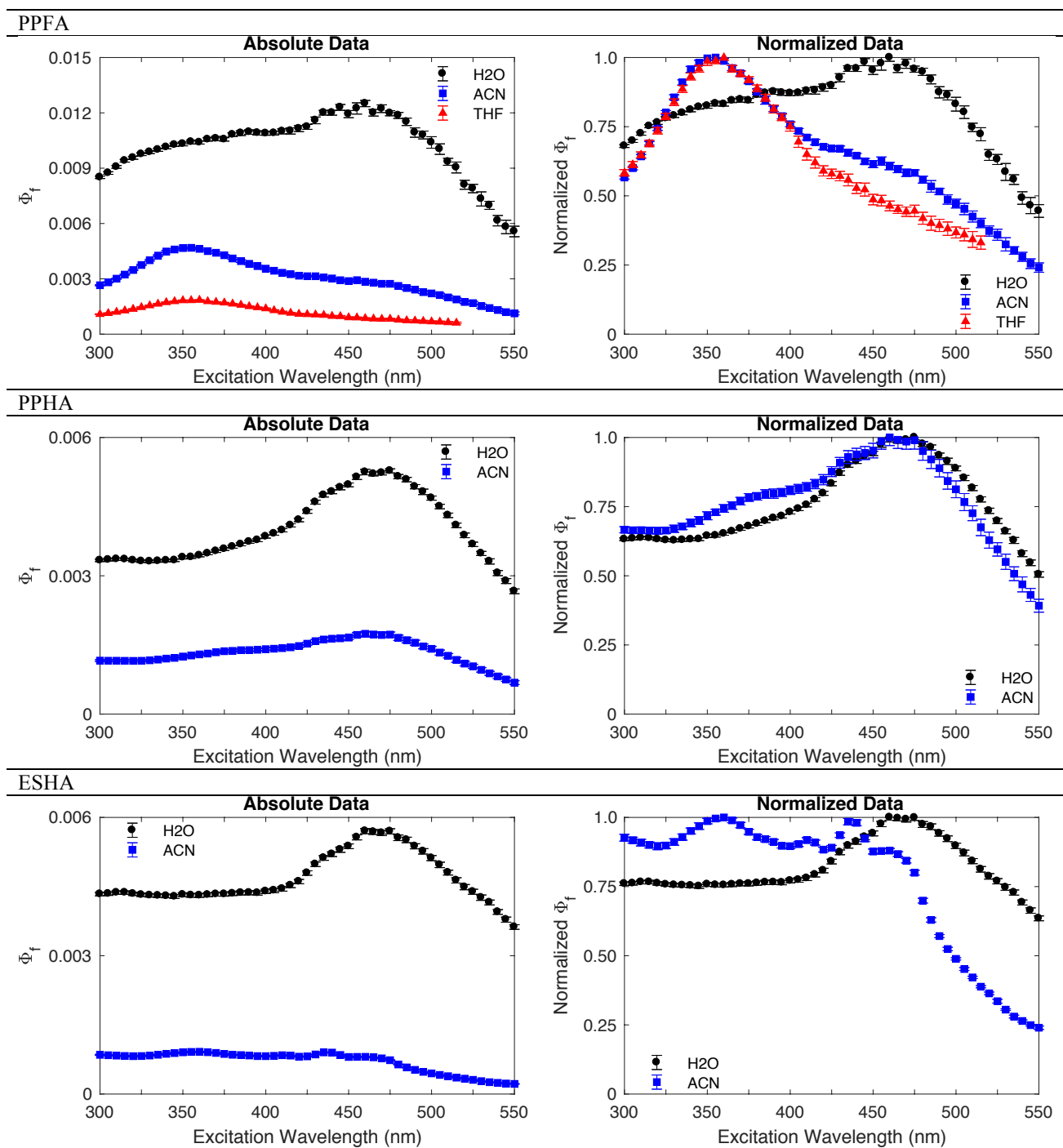
Figure B.19. Effect of solvent on fluorescence quantum yields for PPFA, PPHA and ESHA presented as both measured quantum yields (left pane) and quantum yields normalized to the maximum in each solvent (right pane).
