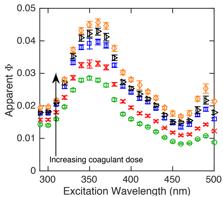
Figure A.8. Apparent fluorescence quantum yields for LM wastewater as a function of increasing alum dose.
