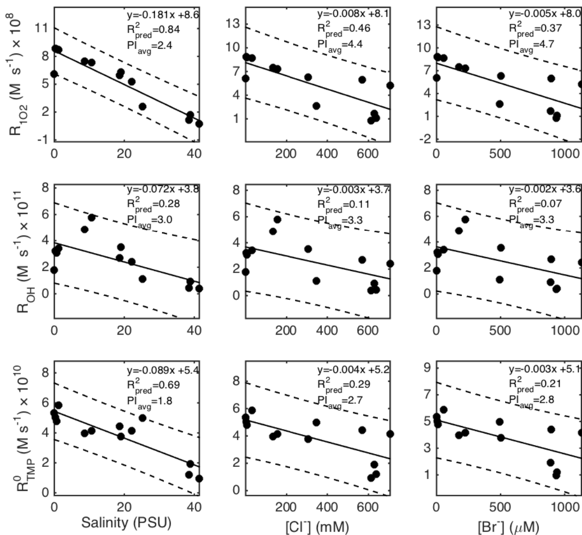
Figure E.13. Relationship between R_{\text{RI}} and salinity for whole water samples. Solid line indicates the model prediction and dashed lines indicate the 95% prediction interval. The fitted model equation and R^2_{\text{pred}} are shown for each prediction-regressor pair. Note that R_{\text{RI}} values for samples with zero salinity (and thus a zero concentration of \text{Cl}^- and \text{Br}^- ) were averaged in the above plot and analyses.
