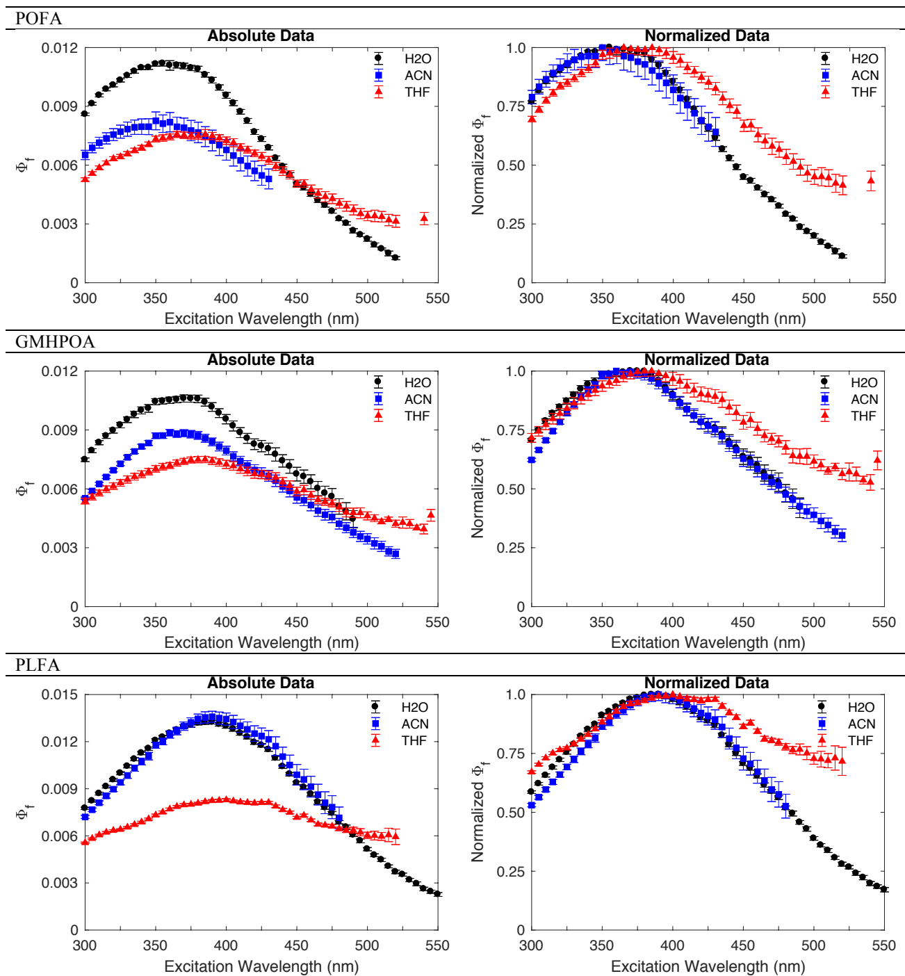
Figure B.16. Effect of solvent on fluorescence quantum yields for POFA, GMHPOA and PLFA presented as both measured quantum yields (left pane) and quantum yields normalized to the maximum in each solvent (right pane).
