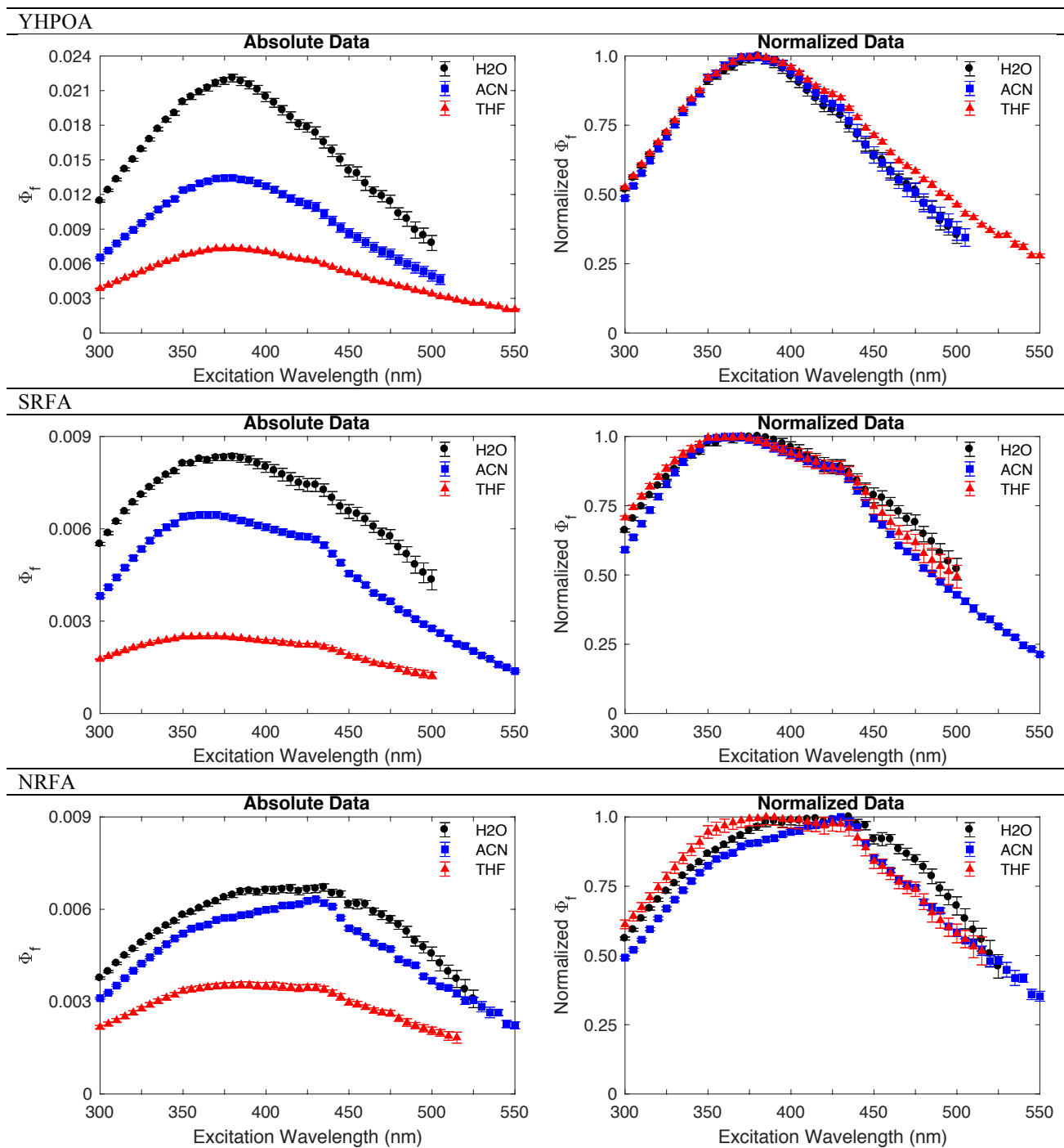
Figure B.18. Effect of solvent on fluorescence quantum yields for YHPOA, SRFA and NRFA presented as both measured quantum yields (left pane) and quantum yields normalized to the maximum in each solvent (right pane).
