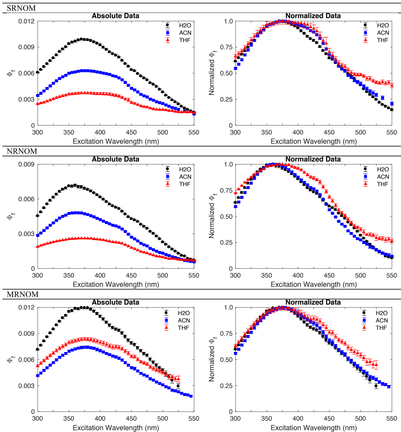
Figure B.17. Effect of solvent on fluorescence quantum yields for SRNOM, NRNOM and MRNOM presented as both measured quantum yields (left pane) and quantum yields normalized to the maximum in each solvent (right pane).
