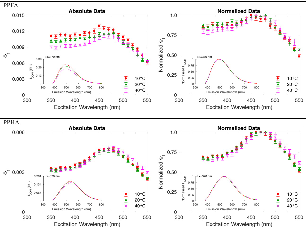
Figure B.5. Effect of temperature on fluorescence quantum yields for PPFA and PPHA presented as both a) measured quantum yields and b) quantum yields normalized to the maximum at each temperature. Inset: emission spectra at an excitation wavelength of 370 nm.
